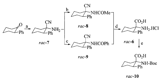
Scheme 2. Synthesis of racemic trans -c 6 Phe and racemic N -Boc trans -c 6 Phe by Strecker reaction: (a) NaCN, NH 4 Cl, i PrOH, NH 4 OH; (b) AcCl, NEt 3 , CH 2 Cl 2 ; (c) BzCl, NEt 3 , CH 2 Cl 2 ; (d) 12 N HCl, reflux; (e) TMAH, acetonitrile, Boc 2 O
