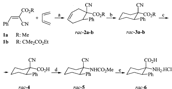
Scheme 1. Synthesis of racemic trans - c 6 Phe by Diels–Alder reaction: (a) Lewis acid (see Table 1), CH 2 Cl 2 , 0 °C; (b) H 2 /Pd/C, EtOH; (c) (i) KOH, EtOH, reflux; (ii) 12 N HCl; (d) (i) PCl 5 , toluene; (ii) NaN 3 , acetone; (iii) toluene, MeOH, reflux; (e) 12 N HCl, reflux
