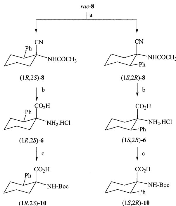
Scheme 3. Synthesis of enantiomerically pure trans -c 6 Phe derivatives: (a) chiral HPLC resolution; (b) 12 N HCl, reflux; (c) TMAH, acetonitrile, Boc 2 O
