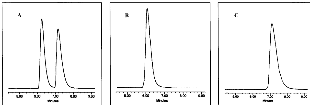
Figure 1. HPLC analytical resolution of acetamide rac -8 (A) and resolved enantiomers (1 R ,2 S )-8 (B) and (1 S ,2 R )-8 (C): column: 150 × 4.6 mm ID containing 3,5-dimethylphenylcarbamate of cellulose (CSP-1); eluent: n -hexane/2-propanol (93:7); flow rate: 1 mL/min; UV detection: 210 nm; chromatographic parameters: k'_1 = 1.53 ; \alpha = 1.24 ; R_S = 1.95
