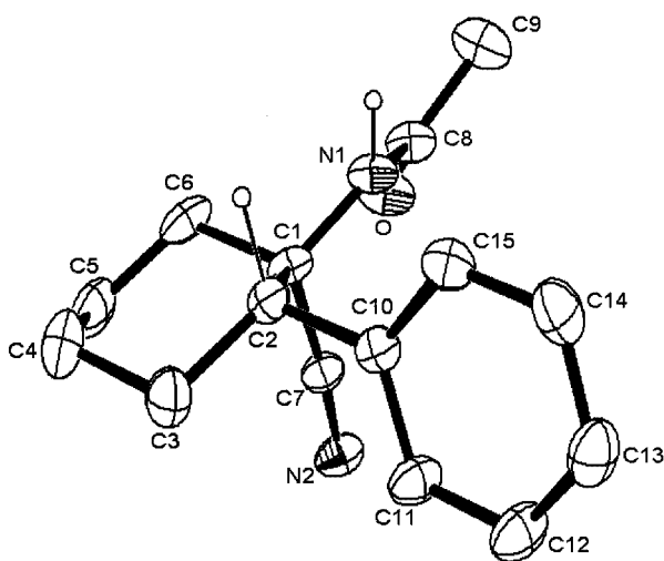
Figure 2. X-ray diffraction structure of (1 R ,2 S )-8 with atom numbering; hydrogen atoms, with the exception of the NH and benzylic protons, are omitted for clarity
